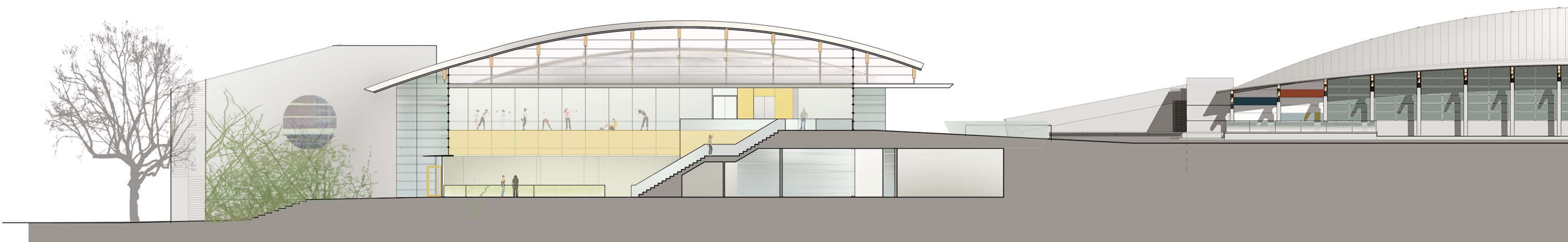
Longitudinal Section Section thru Atrium
