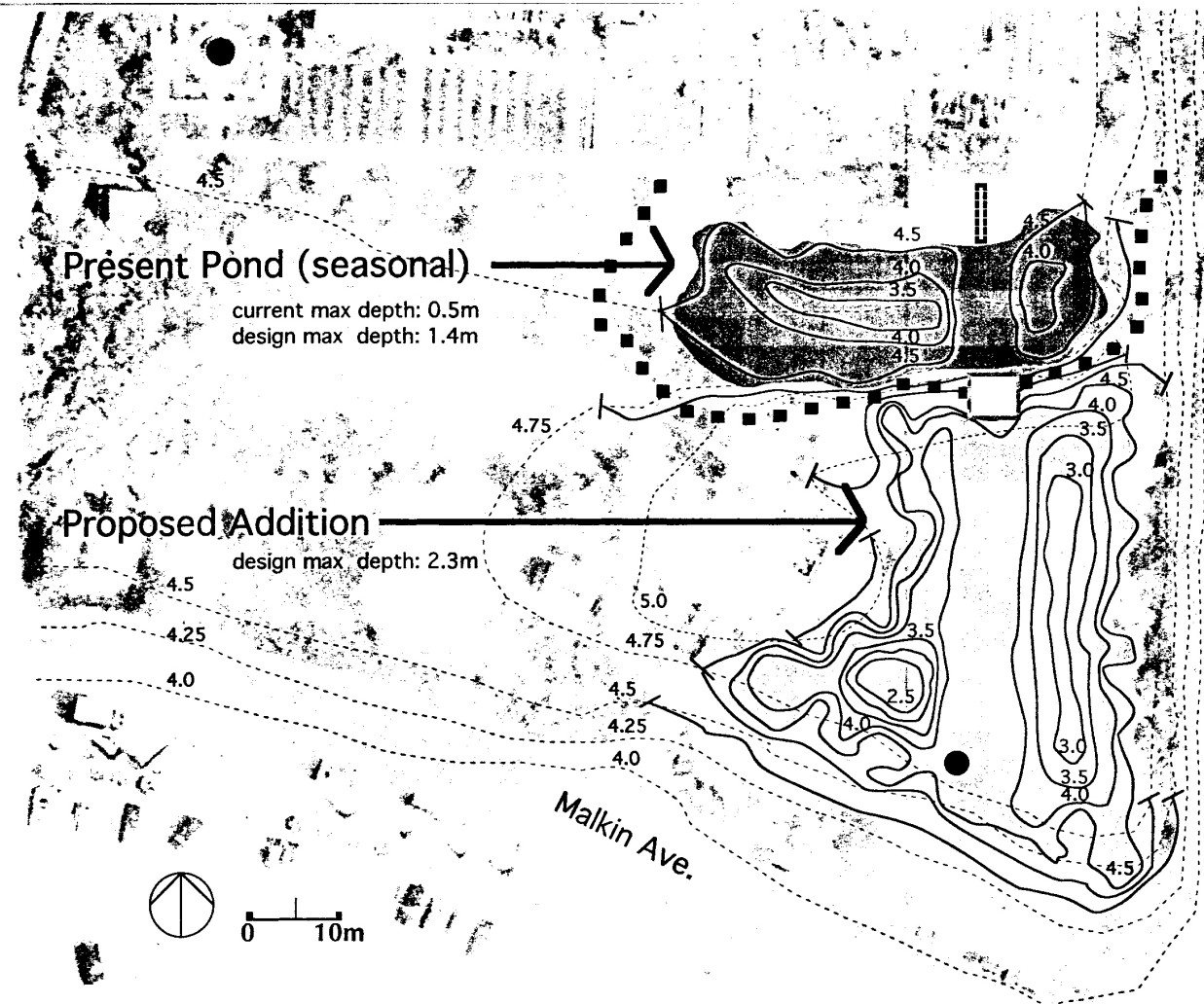
Strathcona Community Gardens Wild Area Project: Grading and Layout Concept
