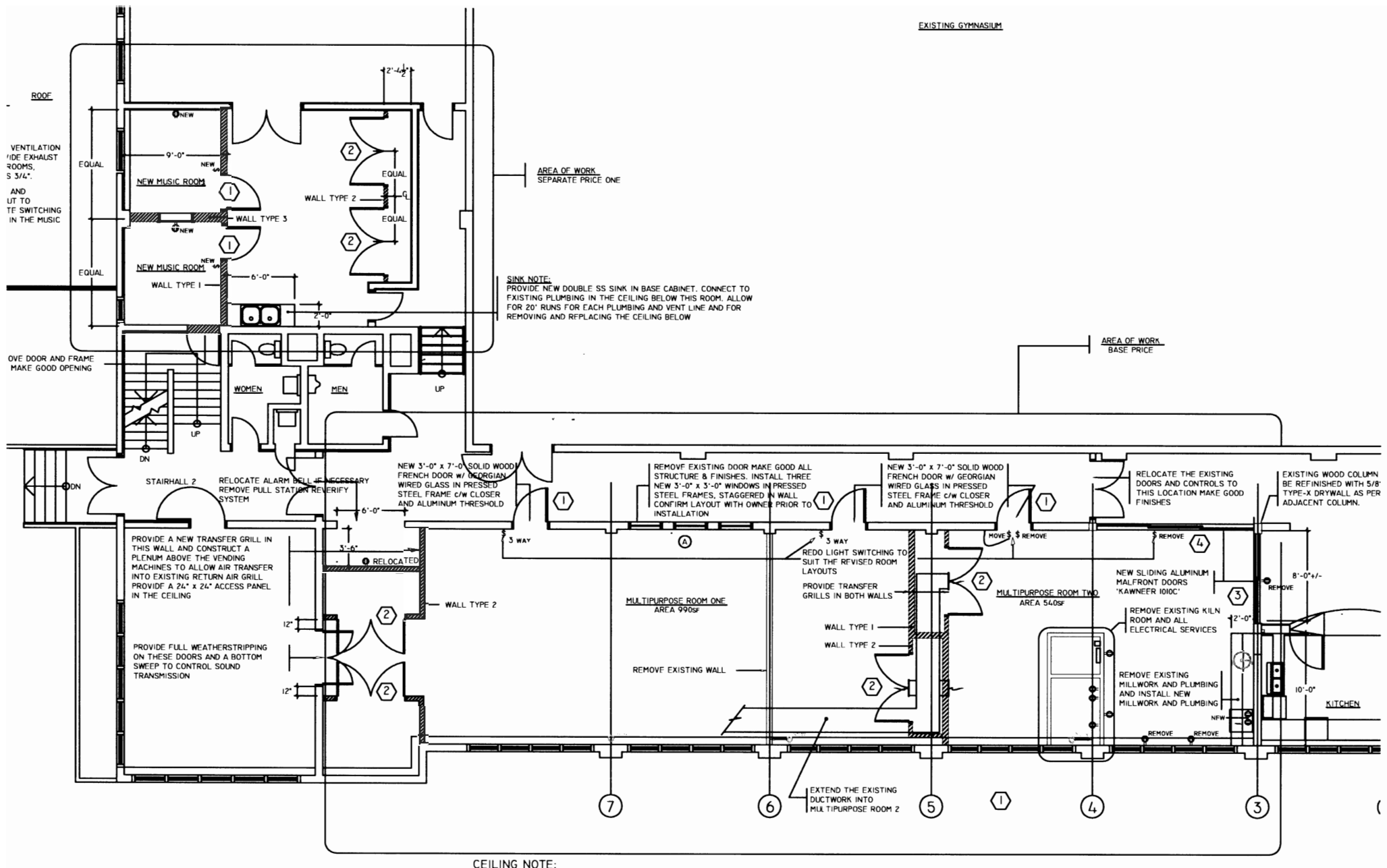
APPENDIX ONE: MARPOLE OAKRIDGE COMMUNITY CENTRE - PROPOSED FLOOR PLAN
